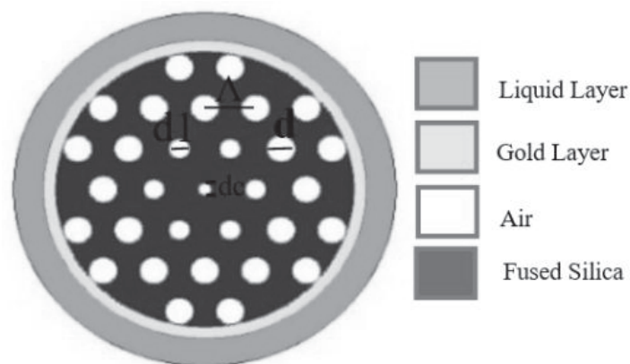
Fig. 1: Cross section view of propounded Sensor
