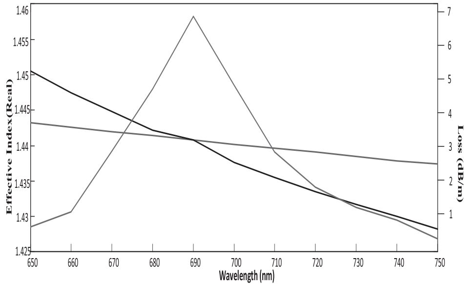
Fig. 3: Relation of dispersion of core mode and surface plasmonpolariton mode
