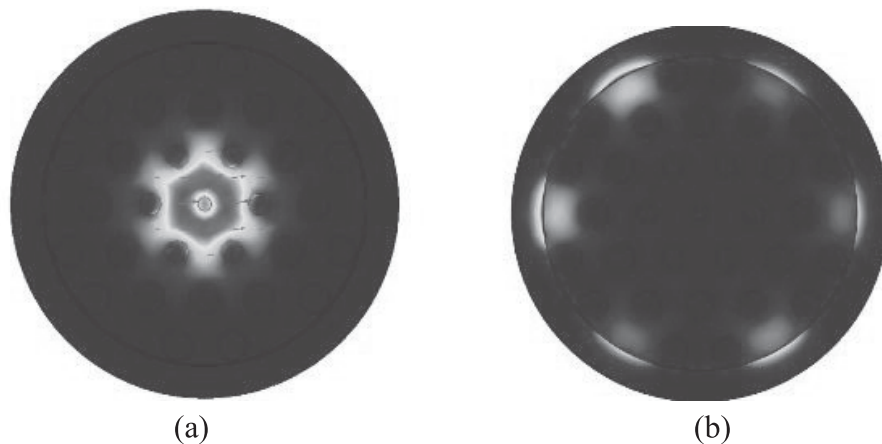
Fig. 2: Field properties of (a) core guided mode for x-polarization and (b) Surface Plasmon Polariton mode
