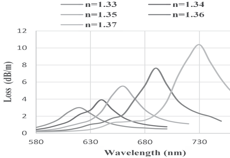
Fig.4: Loss spectrum profile of our proposed sensor by changing analyte RI from 1.33 to 1.3
